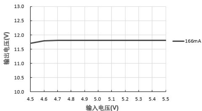
输出电压Vs输入电压 (PS02-B12SS12)
